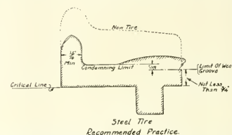
CONDEMNING LIMIT DRAWING FOR STEEL TIED WHEELS, RECOMMENDED FOR INSERTION IN THE INTERCHANGE RULES
