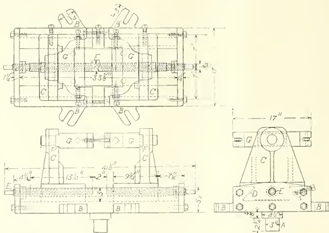
CHUCK FOR MACHINING BACK END OF MAIN ROD BRASSES AND BORING DRIVING BOXES ON BORING MILL
