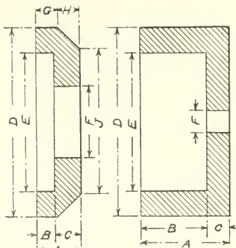
EMERY WHEELS USED FOR AIR BRAKE REPAIRS
