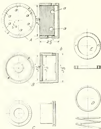
DETAILS OF PNEUMATIC HOLDER-ON.
