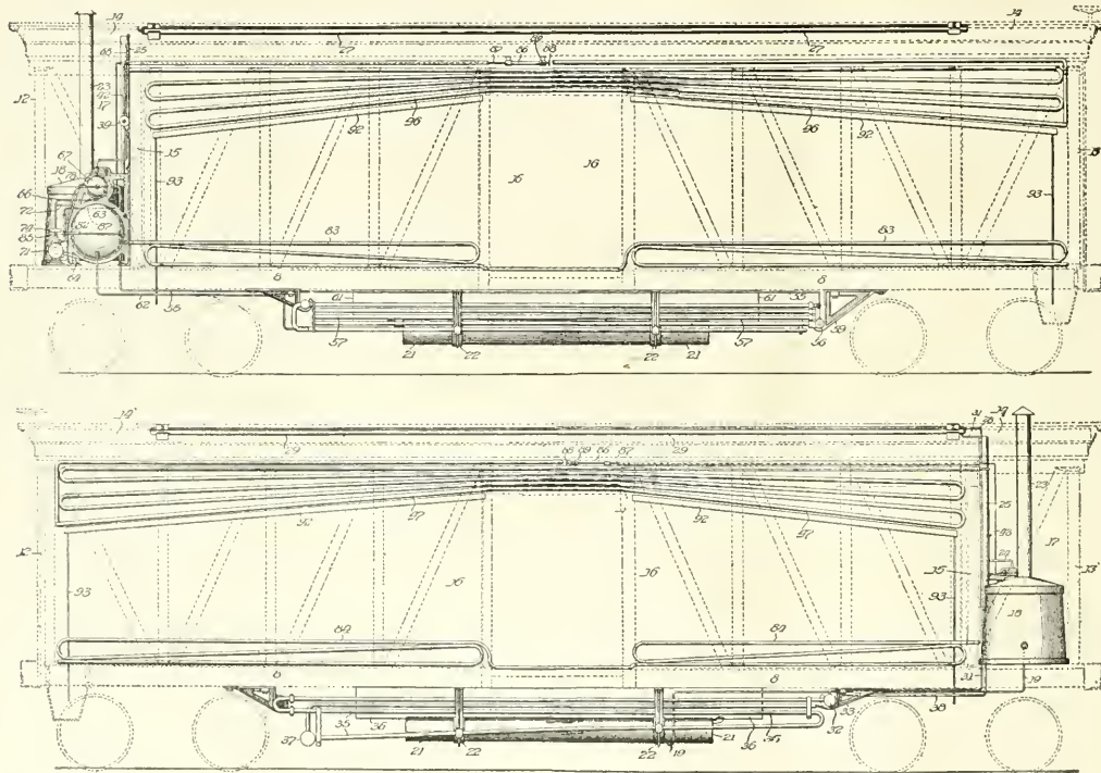
FIG. 3. GENERAL ARRANGEMENT OF APPARATUS OF CAR EQUIPPED WITH AUTHOR'S ABSORPTION REFRIGERATING SYSTEM. (Upper figure shows absorber underneath car; lower figure, of opposite side of car, shows condenser underneath car. Refrigerating coils are shown on upper side walls and heater coils at lower; superheat-dissipating coils on roof of car, operating mechanism at end.)
