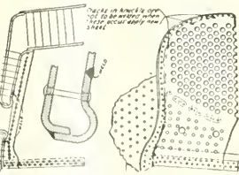
FIG. 18. KNUCKLE CRACKS NOT TO BE WELDED.
