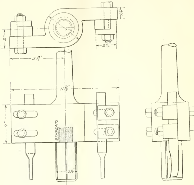
TOOL FOR BORING SIDE ROD BUSHINGS
