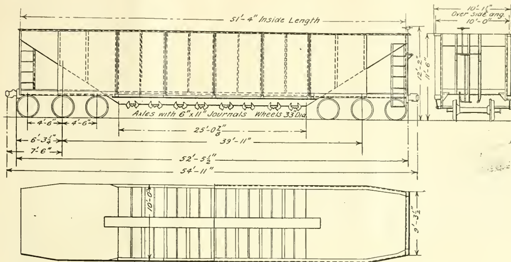
GENERAL OUTLINES, 240,000 LBS. CAPACITY COAL CAR
