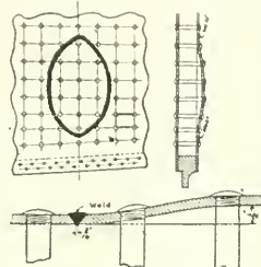
FIG. 8. PATCHING AROUND DEFECTIVE STAYBOLTS.
