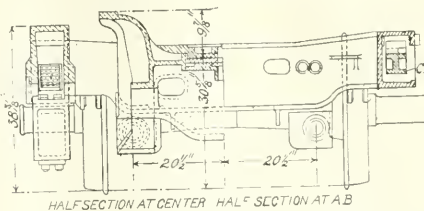
SIX WHEEL COMMONWEALTH STEEL TENDER TRUCK FOR DENVER & RIO GRANDE MOUNTAIN LOCOMOTIVE
