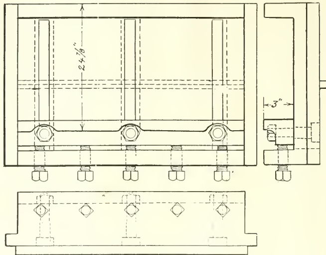
CHUCK FOR PLANING SHOES AND WEDGES.
