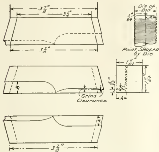
DIES FOR POINTING STAYBOLTS.
