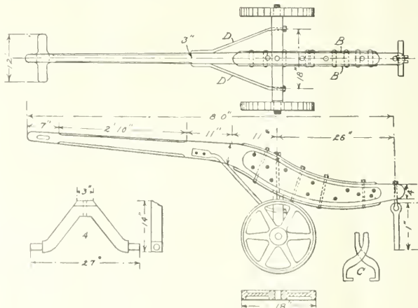
ROD TRUCK.
