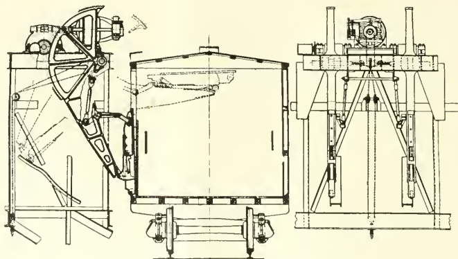
DOOR OPENER ARRANGEMENT OF UNLOADER
