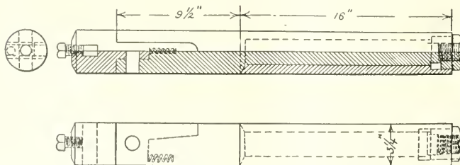
DETAILS OF KNUCKLE TOOL HOLDER FOR SLOTTOR
