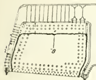
FIG. 6. THE KNUCKLE PATCH IN THE FIREBOX.
