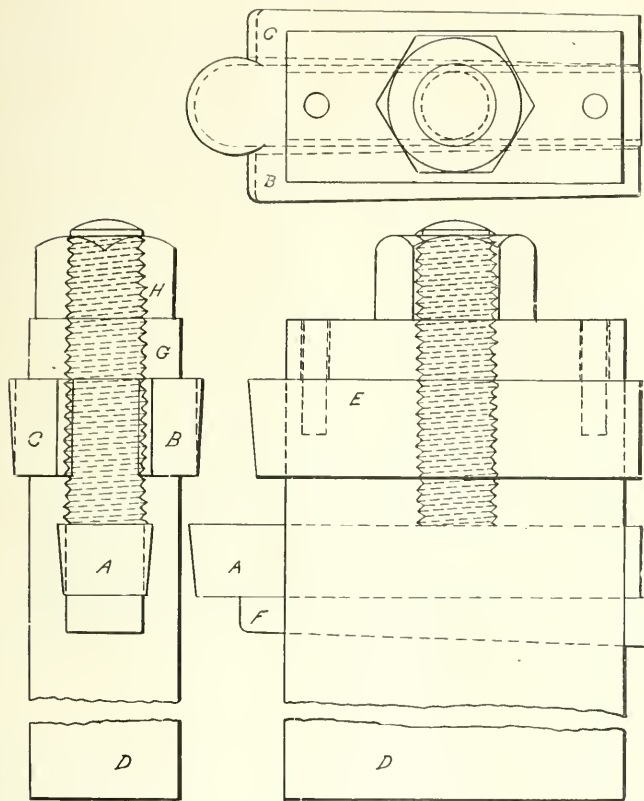
TOOL POST FOR SLOTTOR
