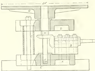
DRY PIPE GRINDING APPARATUS
