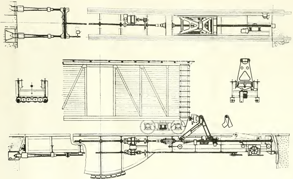
BUMPER AND LOCK ARRANGEMENT OF UNLOADER
