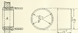
STEEL THIMBLE FOR PROTECTING BOILER TUBES
