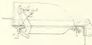
DROP DOOR LATCH, NORFOLK & WESTERN R. R. 120-TON CAR
