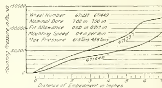
FIG. 2. AUTOGRAPHIC DIAGRAMS OF PRESSURES REQUIRED TO MOUNT TWO 33-IN. 725-LB. WHEELS ON AXLE
