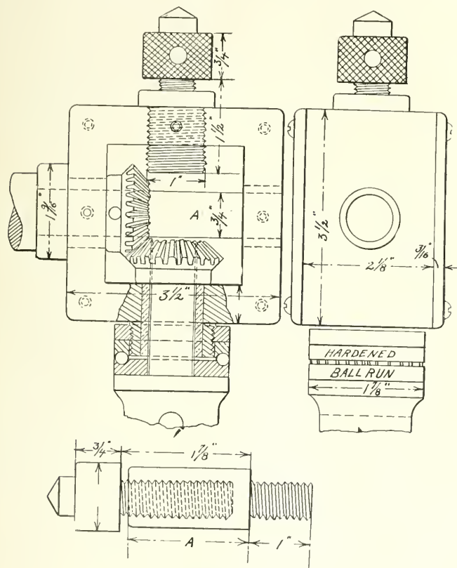
RIGHT ANGLE DRILL.
