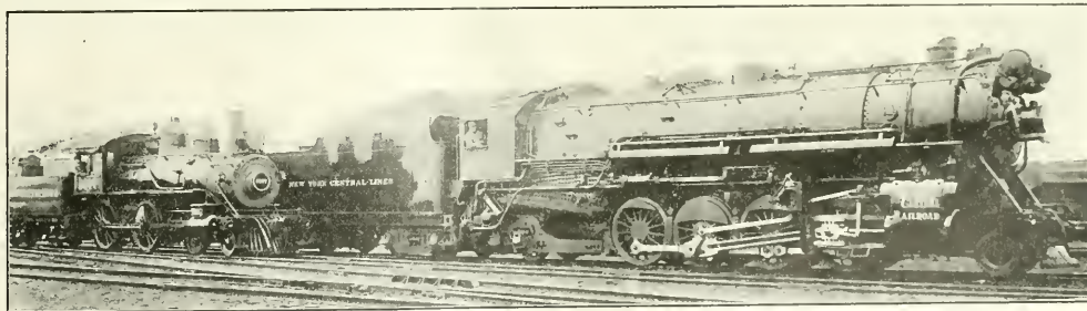
MIKADO 2-8-2 TYPE LOCOMOTIVE NO. 8000, OF THE MICHIGAN CENTRAL, SAID TO BE THE MOST POWERFUL OF ITS WEIGHT AND ON THE LEFT, ENGINE NO. 8977, FORMERLY 248, STILL RUNNING AFTER A SERVICE OF FORTY YEARS
