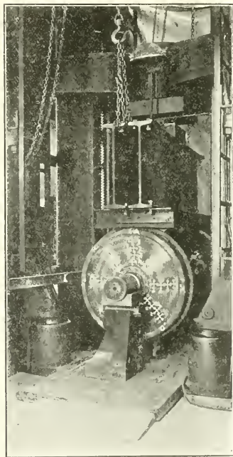
600,000-LB. TESTING MACHINE WITH PAIR OF WHEELS IN POSITION TO RECEIVE STATIC LOAD
