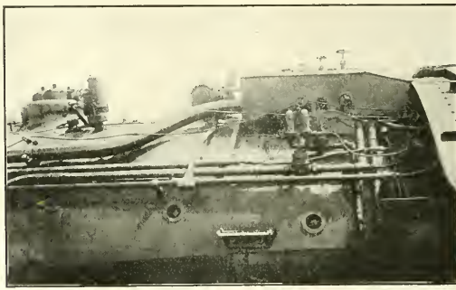
VIEW OF LOCOMOTIVE NO. 8000, SHOWING STEAM TURRET ON TOP OF BOILER IMMEDIATELY IN FRONT OF CAB
