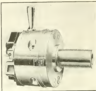
\frac{5}{8} IN. AND \frac{7}{8} IN. AUTOMATIC HEAD
