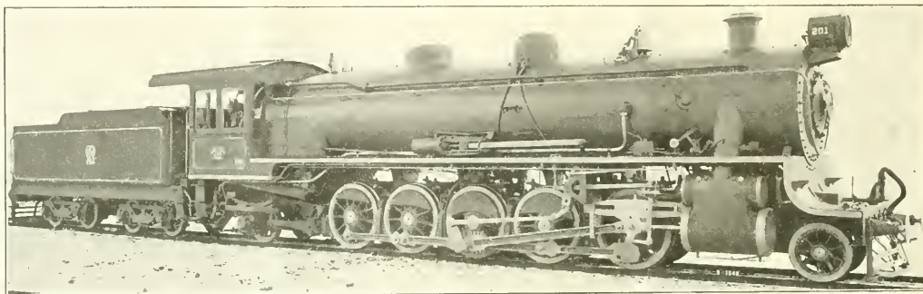
SANTA FE 2402 TYPE LOCOMOTIVE FOR THE MANILA RAILROAD. AMERICAN LOCOMOTIVE COMPANY, BUILDERS.
