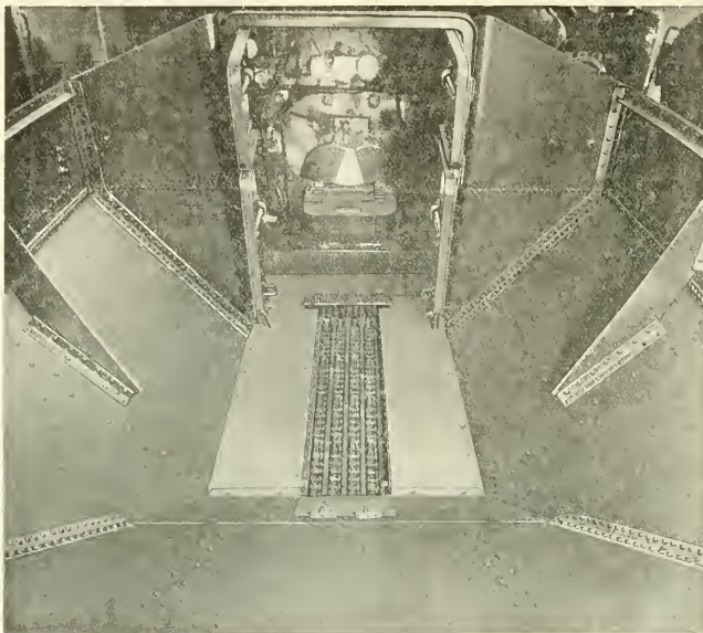
Elvin Stoker Installation on a Recent Heavy Mountain Type Locomotive
