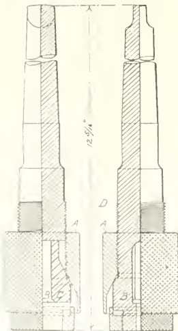
CHUCK FOR FLAT DRILLS.
