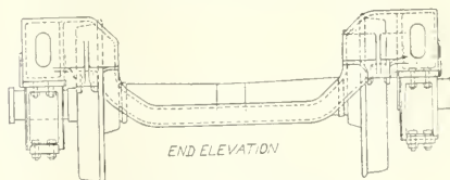
SIX WHEEL TENDER TRUCK
