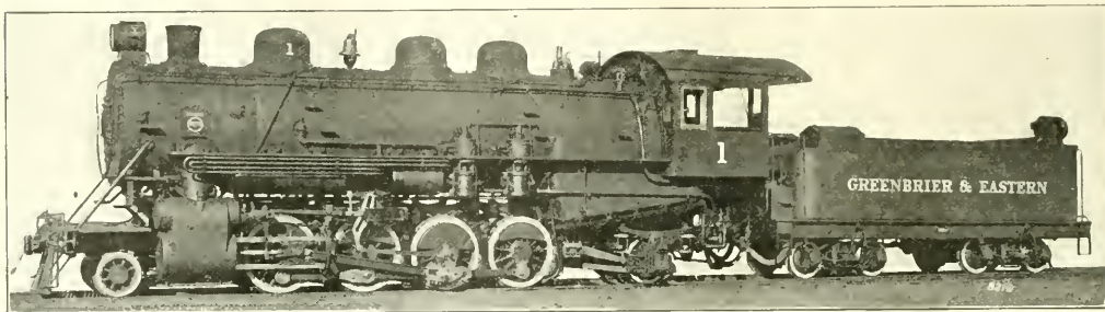
MIKADO TYPE 2-8-2 LOCOMOTIVE FOR THE GREENBRIER & EASTERN RAILROAD, BALDWIN LOCOMOTIVE WORKS, BUILDERS
