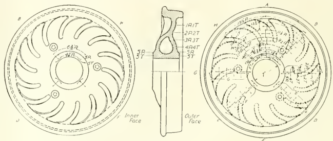
FIG. 1. LOCATION OF GAGE-LINES ON 33-IN. 725-LB. M. C. B. WHEEL NO. 671,237
