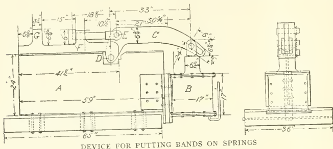
DEVICE FOR PUTTING BANDS ON SPRINGS
