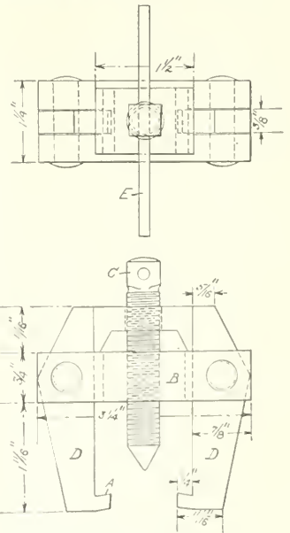
CLAMP FOR SAFETY VALVE IN HYDROSTATIC TESTS
