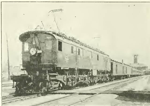
THE OLYMPIAN DRAWN BY BALDWIN-WESTINGHOUSE LOCOMOTIVE LEAVING BUTTE, MONTANA, STATION
