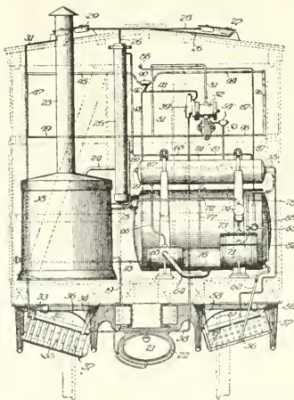
FIG. 1. CAR REFRIGERATING SYSTEM
