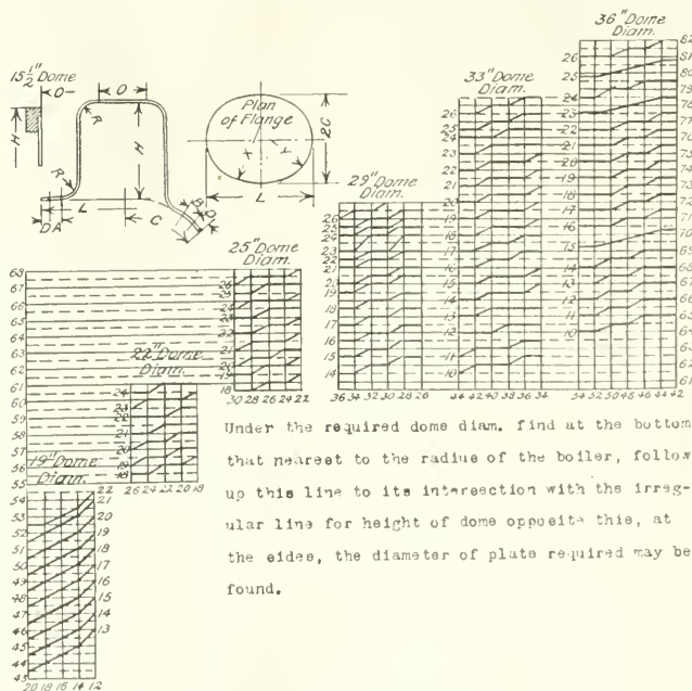
METHOD OF DETERMINING OR FINDING SIZES OF PLATES FOR PRESSED STEEL DOMES (BALDWIN LOCOMOTIVE WORKS).
