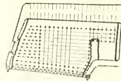
FIG. 5. FIREBOX AND COMBUSTION CHAMBER WELDED.
