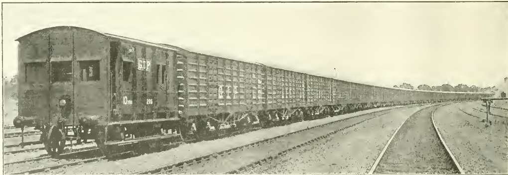
FIG. 2. 2,000 TON TRAIN, VIEW FROM REAR TO SHOW 10-TON CABOOSE. TRAIN THROUGHOUT FITTED WITH CONTINUOUS BRAKES
