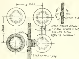
FIG. 7. HOW CRACKS AT STAY-BOLT HOLES ARE WELDED.
