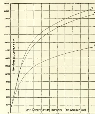
COMPOSITE STRESS - STRAIN CURVES OBTAINED FROM TENSILE TESTS ON SAMPLES OF WHEELS OF THE THREE MANUFACTURERS
