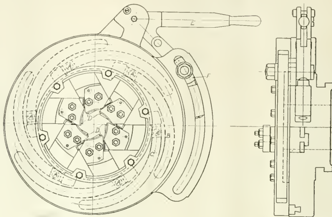
DIE HEAD OF THE LANDIS 12-INCH PIPE CUTTING AND THREADING MACHINE.
