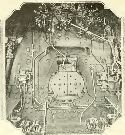
THE FRANKLIN AUTOMATIC FIREDOOR BUTTERFLY TYPE
