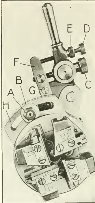
NEW DIE HEAD WITH MICROMETER ATTACHMENT.
