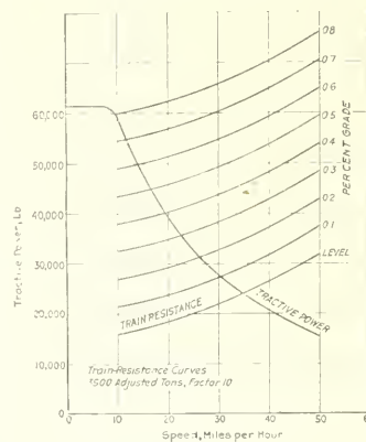
TRACTIVE POWER-SPEED AND TRAIN-RESISTANCE CURVES
