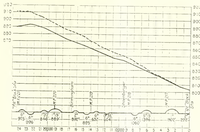
PORTION OF A RAILROAD BETWEEN BLOCK SECTIONS QY AND FR
