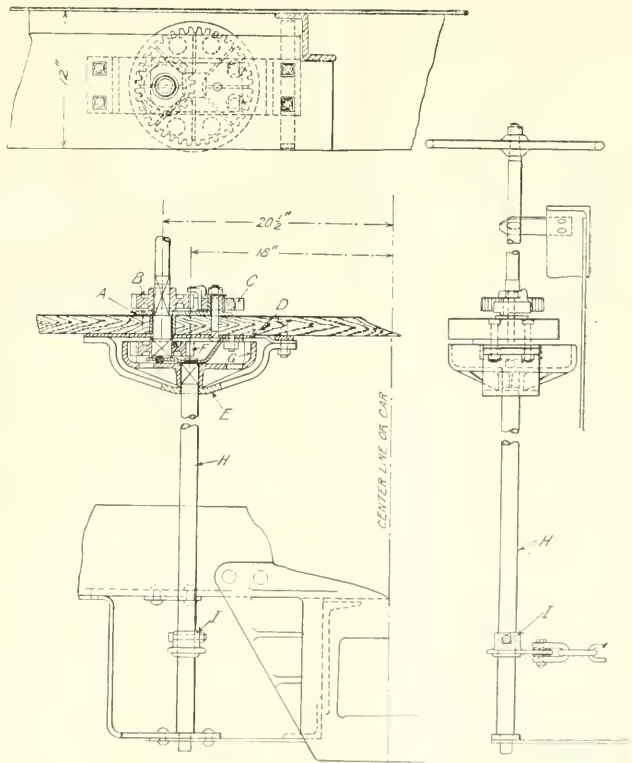
HAND BRAKE STAFF, 240,000 LBS. CAPACITY COAL CAR
