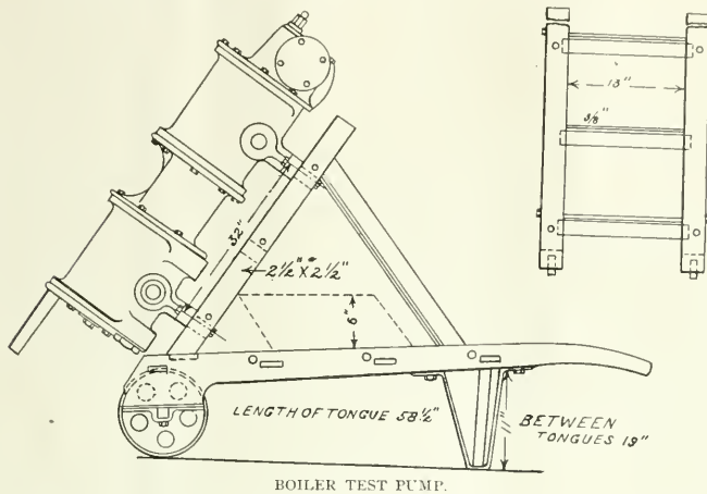
BOILER TEST PUMP.
