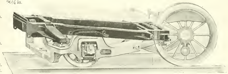
DELTA TRUCK USED ON MOUNTAIN TYPE LOCOMOTIVE
