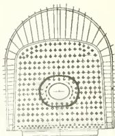
FIG. 17. PATCH WELDED ON DOOR COLLAR.
