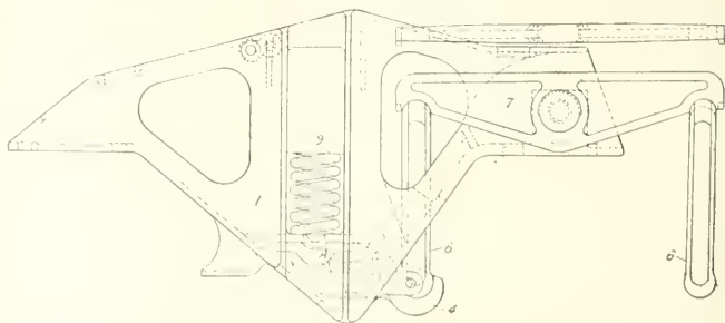
ASSEMBLY OF DETAILS FOR LOAD TRANSFERENCE, NORFOLK & WESTERN RY. TRUCK
