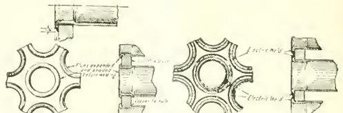
FIG. 19. USE THIS METHOD OF APPLYING FLUES IN LOCOMOTIVE BOILERS BY MEANS OF THE ELECTRIC ARC WELDING PROCESS.
