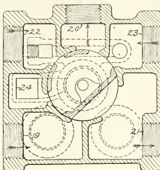
FIG. 6. CUT-OUT VALVE, SHUT OFF POSITION.
