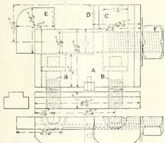
HEAVY DUTY CHUCK FOR BORING MILL
