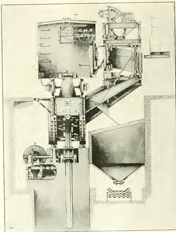
GENERAL ARRANGEMENT OF BOX CAR UNLOADER FOR GRAIN
