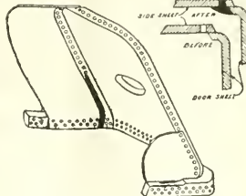
FIG. 15. METHOD OF WELDING DEFECTIVE SEAMS.
