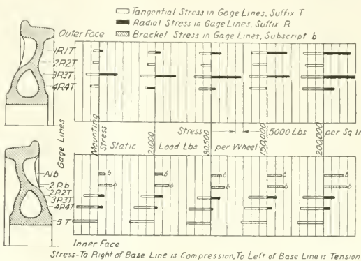
FIG. 4. CORRESPONDING SIMPLE UNIT STRESSES IN 33-IN. 725-LB. M. C. B. WHEEL NO. 671,449 DUE TO COMBINED EFFECTS OF MOUNTING AND STATIC LOADS. LOADS APPLIED ON THE A RADIAL.
