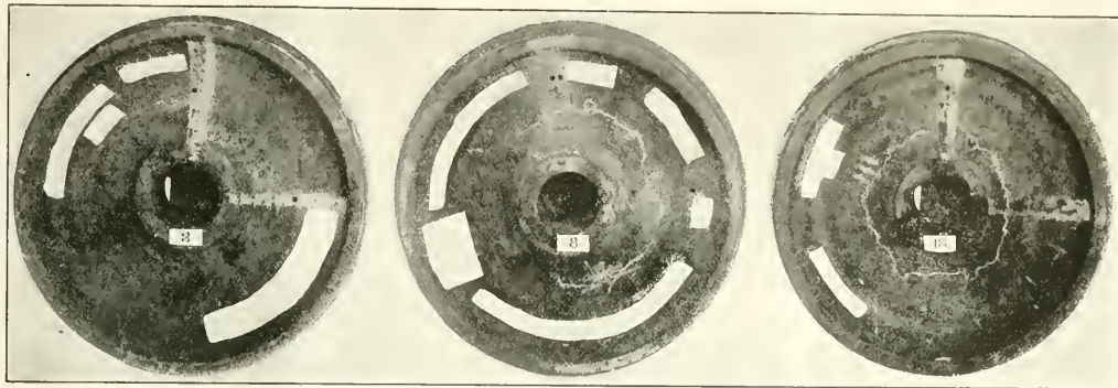
WHEELS FAILING UNDER THERMAL TESTS SHOWING CRACKS
