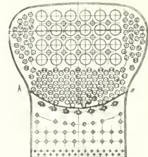
FIG. 13. TOP PORTION OF BACK FLUE SHEET AS ARRANGED NEW FOR SUPERHEATER.
