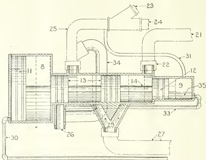
ROBERTS DRIFTING VALVE IN DRIFTING POSITION.
