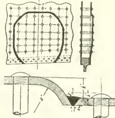
FIG. 9. PATCH IN SIDE SHEET.
