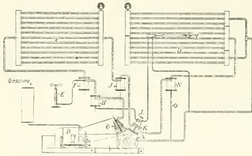
FIG. 4. DIAGRAM SHOWING PROCESS EMPLOYED ON MOTOR TRUCK.
