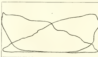
TYPICAL EXAMPLES OF INDICATOR CARDS TAKEN ON ROAD TESTS
