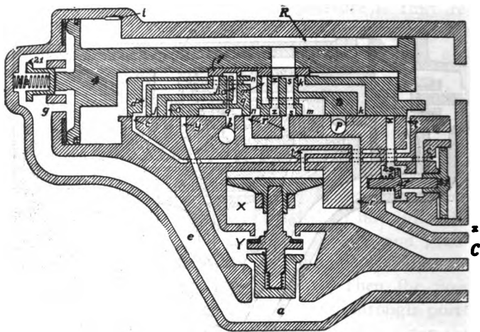
FIG. 356. EMERGENCY POSITION
