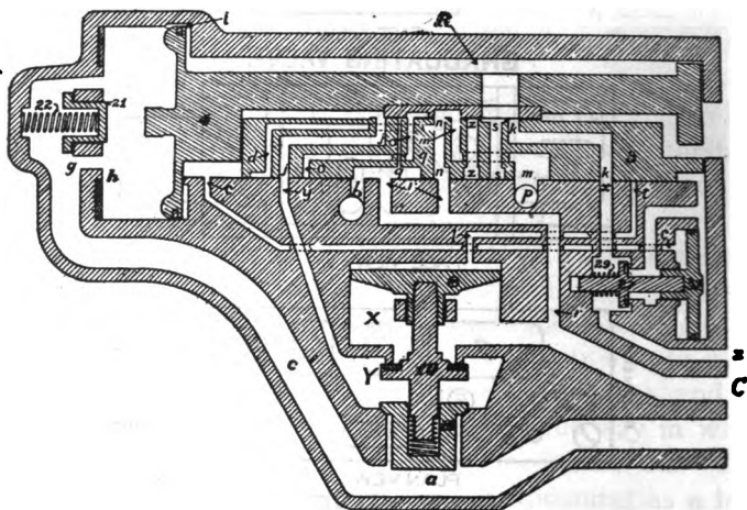
FIG. 351. FULL RELEASE AND CHARGING POSITION
