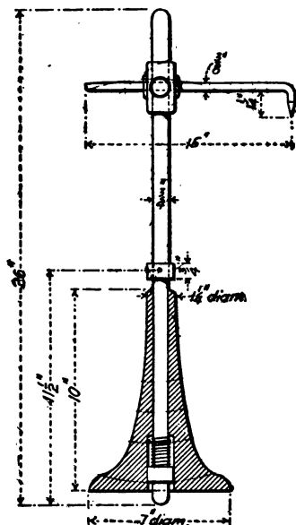
FIG. 338. A CONVENIENT GAUGE FOR SETTING THE ECCENTRIC CRANK
