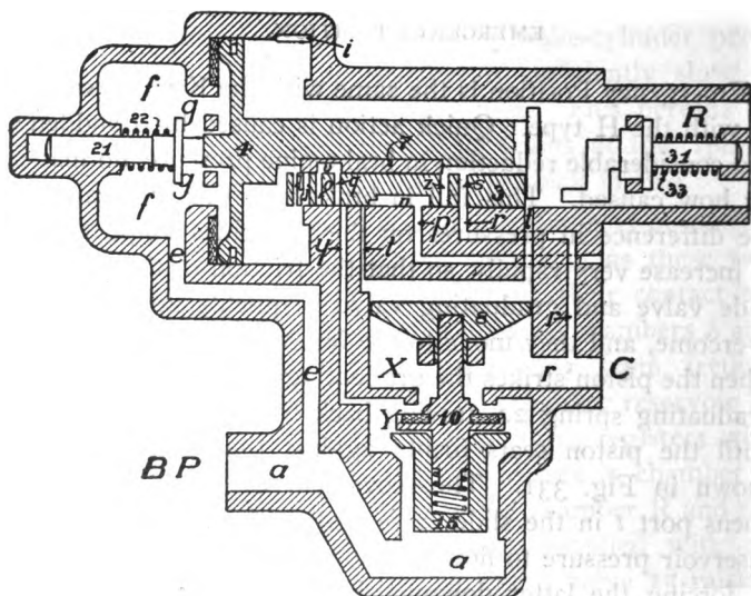
.FIG. 331. EMERGENCY POSITION
