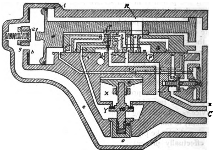
FIG. 354. SERVICE-LAP POSITION
