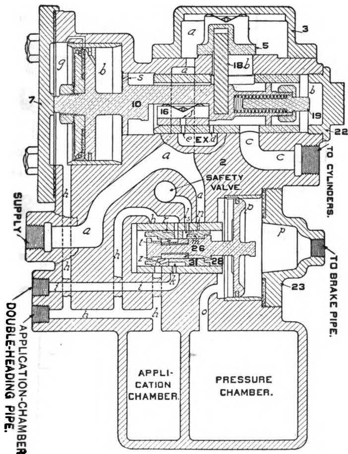
FIG. 306. RELEASE POSITION
