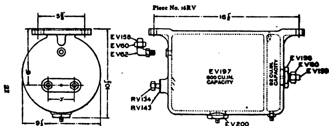
Fig. 279. Divided Reservoir.
