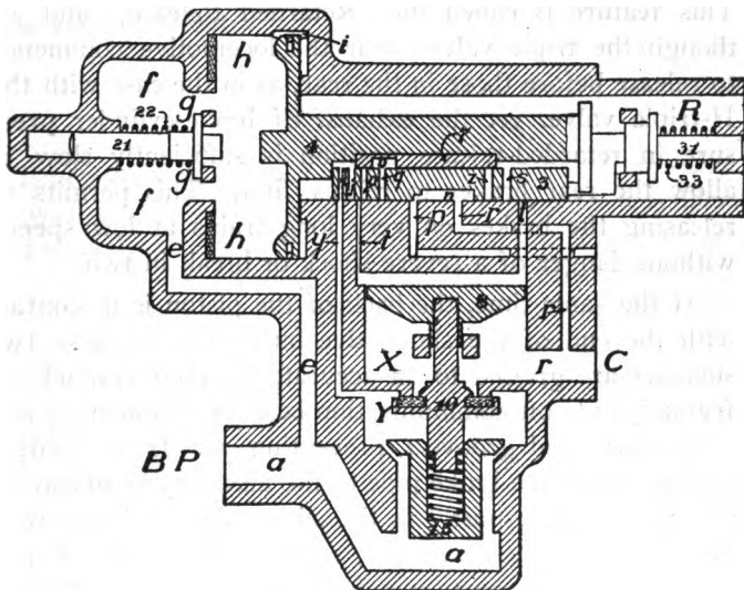
FIG. 330. RETARDED-RELEASE POSITION.
