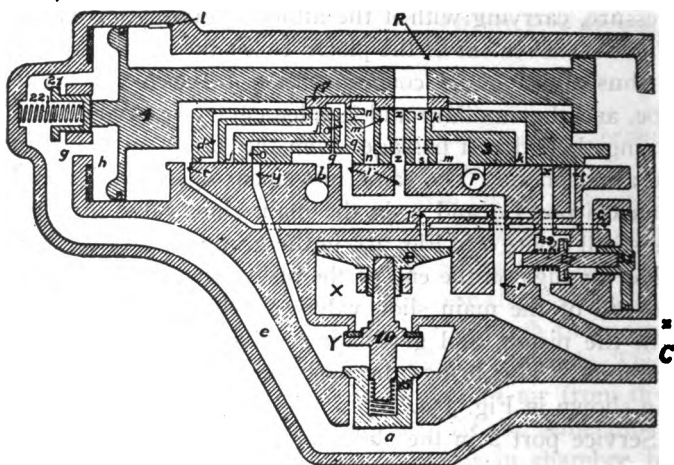
FIG. 353. FULL-SERVICE POSITION
