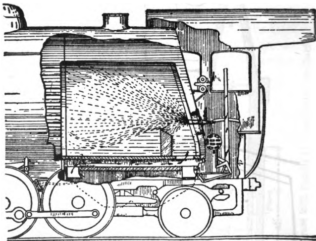
Figure 223k. Lasso-Lovekin Oil-Burner. Dispenses with Brick Arch. Oil Supplied Under Pressure.
