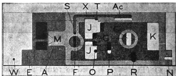
Fig. 273. Running Position.
