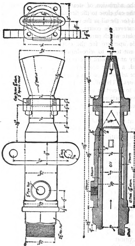
Figure 2281. Details of "Lundholm" Oil-Burner.
