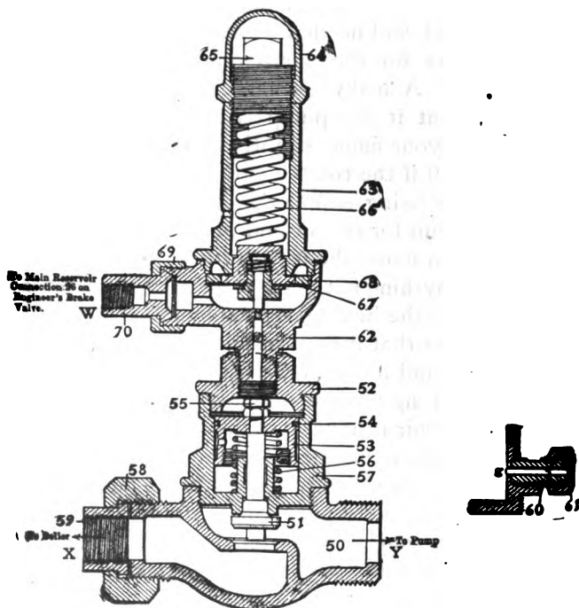
FIGURE 226 PUMP GOVERNOR
