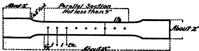
TEST PIECE
