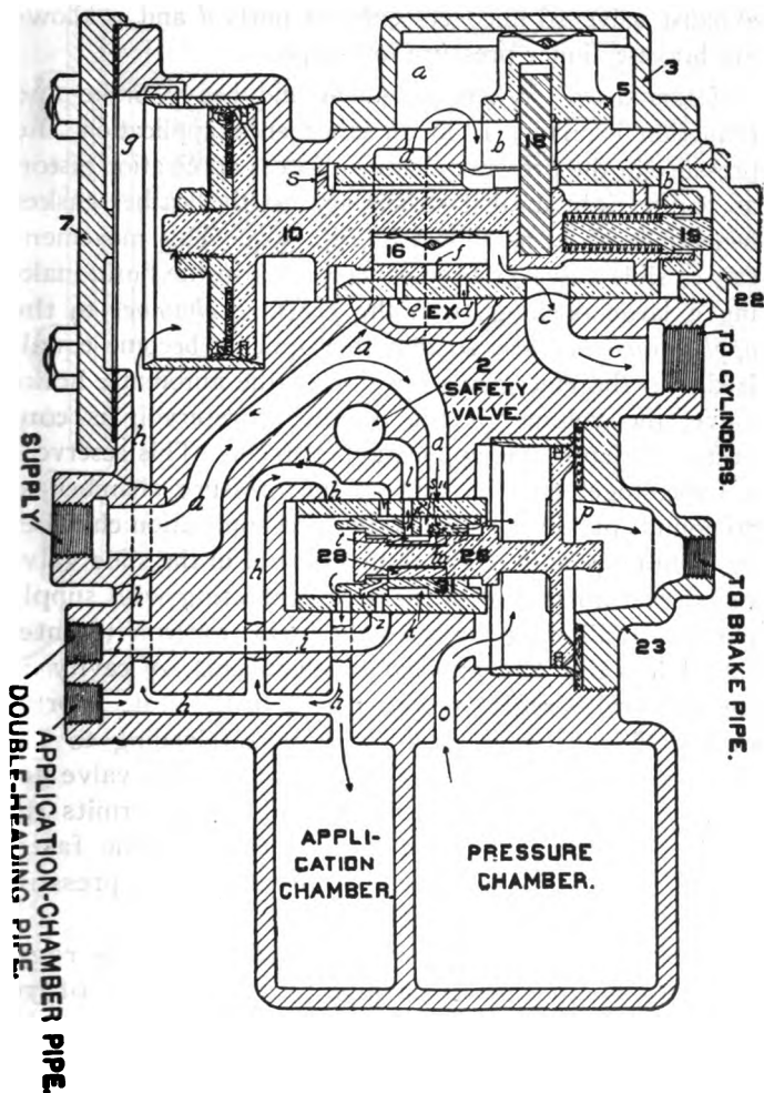
FIG. 304. EMERGENCY
