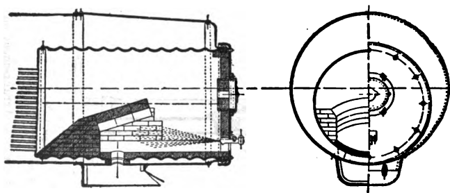
Figure 223m. Oil-Burner in Vanderbilt Type of Firebox.
