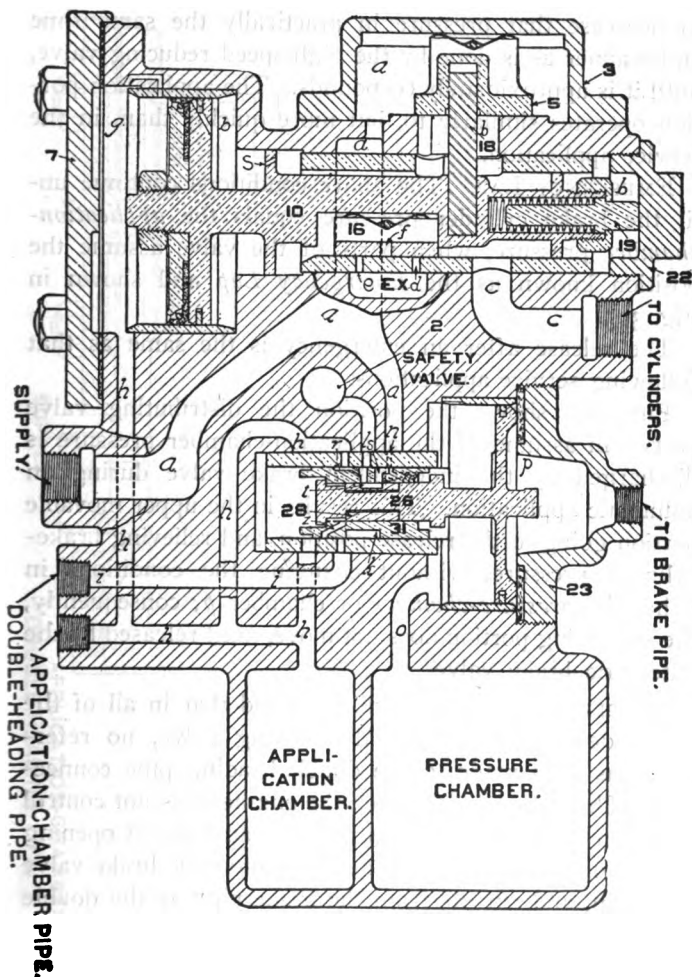
FIG. 305. EMERGENCY LAP
