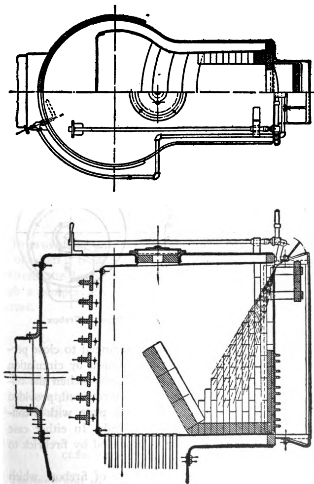
Figure 223 I. Burner and Firebox Arrangement on Baldwin Locomotive.
