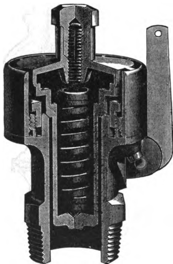
FIGURE 194 KUNKLE POP VALVE FOR PORTABLE AND STATIONARY BOILERS
