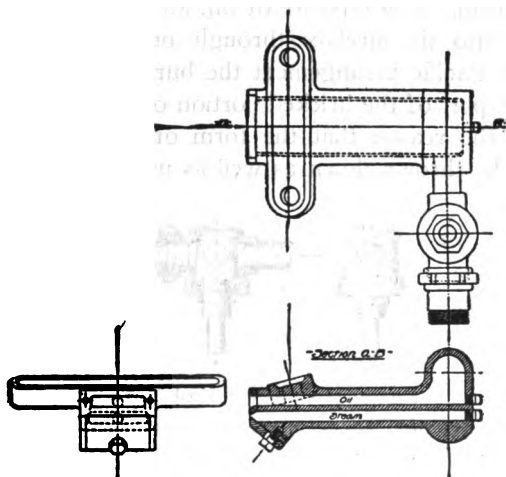
Figure 233g. Baldwin Oil-Burner.
