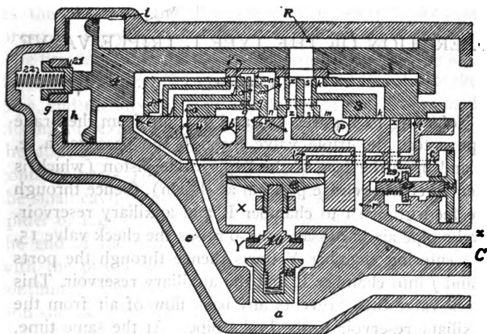
FIG. 352 QUICK-SERVICE POSITION
