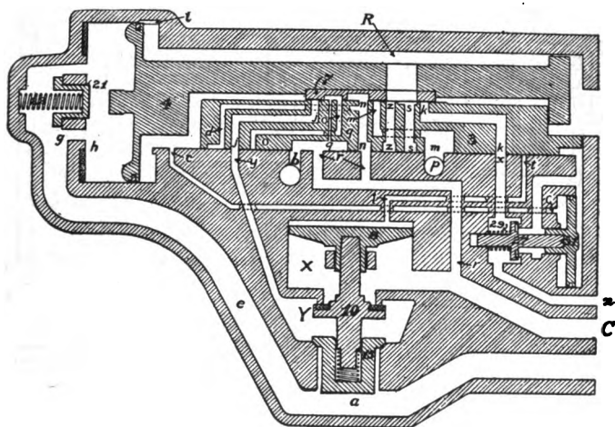
FIG. 355. GRADUATED-RELEASE-LAP POSITION
