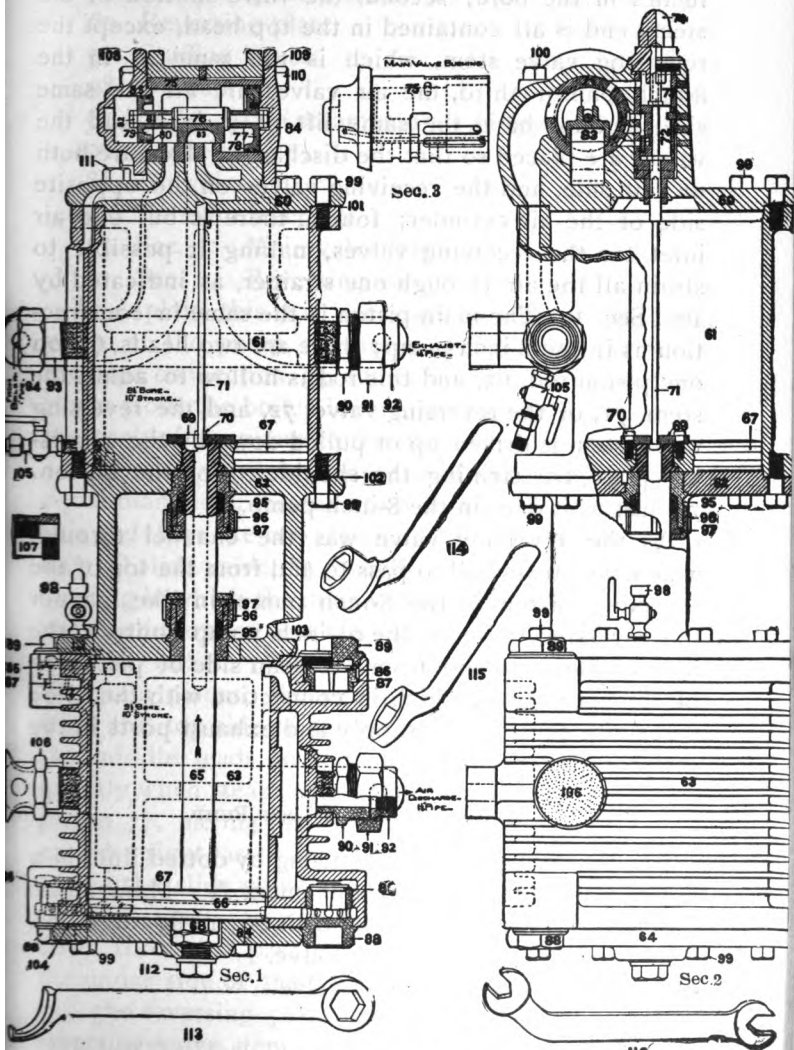
FIGURE 225 NINE AND ONE-HALF INCH PUMP — See page 520.
