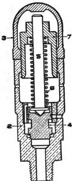
FIG. 309. SAFETY VALVE
