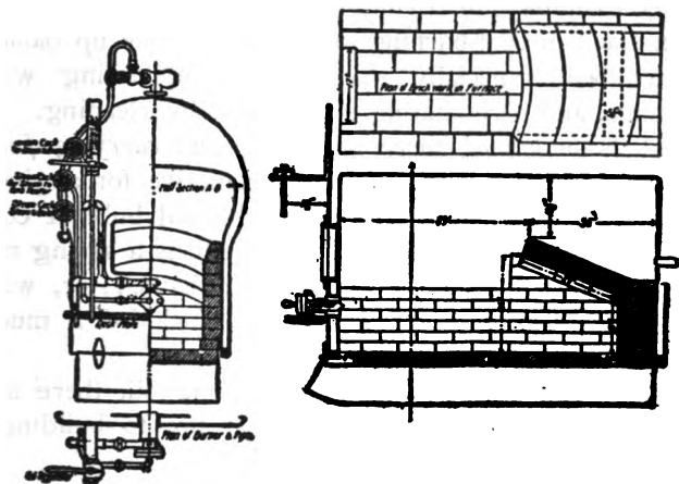
Figure 223a. Details of Oil-Burning Furnace.
