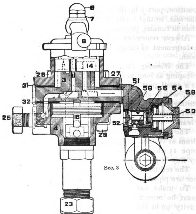
FIGURE 231 G-6 BRAKE VALVE
