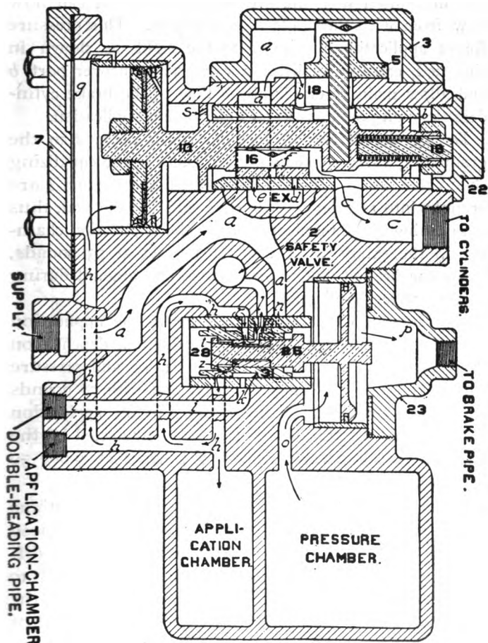
FIG. 302. AUTOMATIC SERVICE
