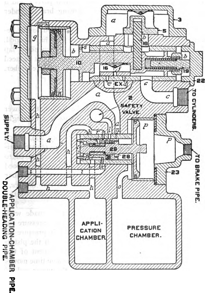
FIG. 301. INDEPENDENT LAP
