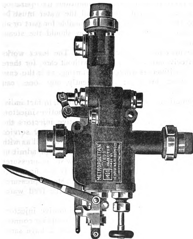
FIGURE 163 METROPOLITAN "1898" LOCOMOTIVE INJECTOR
