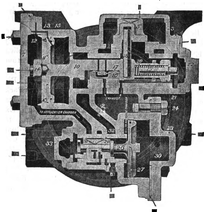
FIG. 308. DISTRIBUTING VALVE
