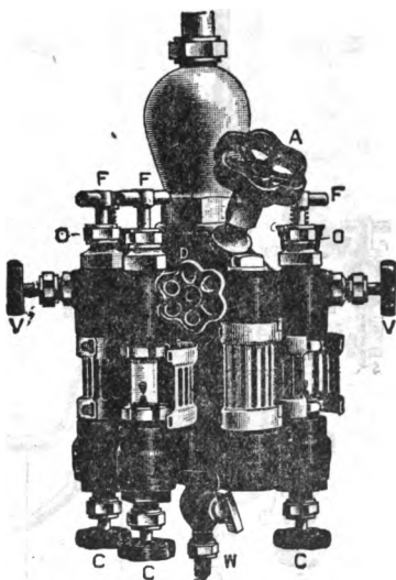
FIGURE 198 NEW NATHAN LUBRICATOR, FRONT VIEW
