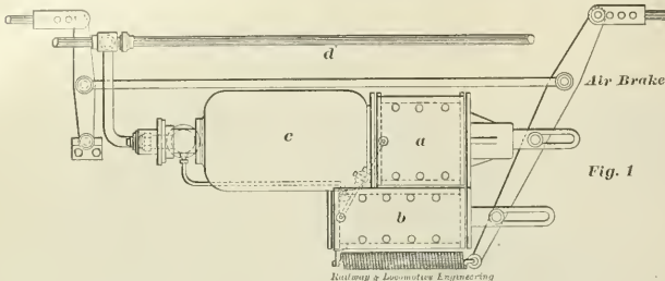
A REINFORCED BRAKE.
