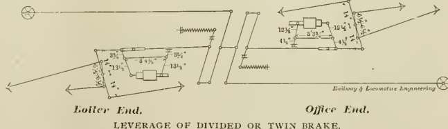
LEVERAGE OF DIVIDED OR TWIN BRAKE.
