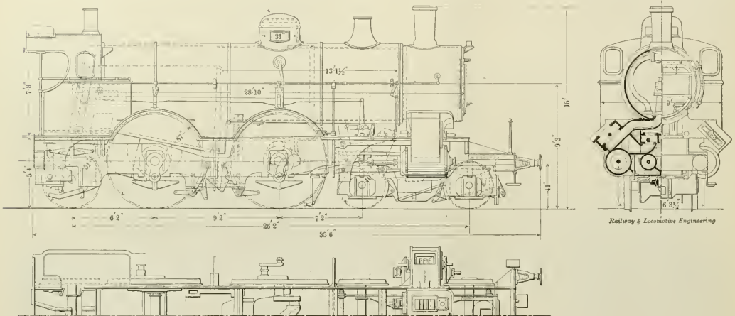
DETAILS OF FOUR CYLINDER COMPOUND ON THE AUSTRIAN STATE RAILWAY.
