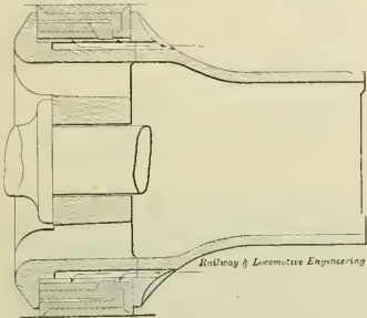
FIG. 14. "AMERICAN" ONE RING COMPLETE.
