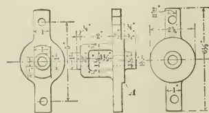
DETAILS OF A HANDY TOOL FOR AIR BRAKE WORK.
