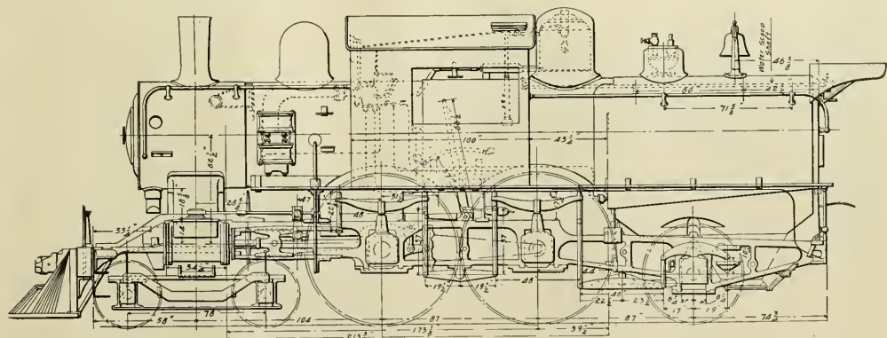
ATLANTIC LOCOMOTIVE ELEVATION-CENTRAL RAILROAD OF NEW JERSEY.
