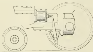
FIG. 1—BRAKE CYLINDER LOCATION.
