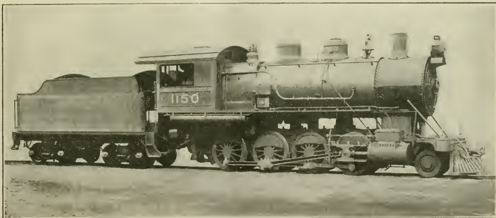
ROGERS CONSOLIDATION FOR GREAT NORTHERN.
