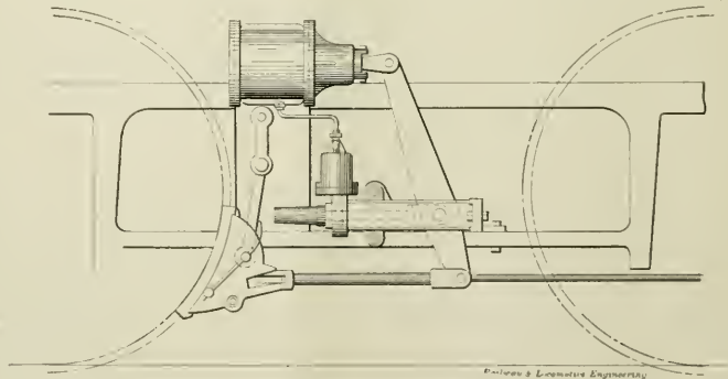
SLACK ADJUSTER ON DRIVER BRAKES
