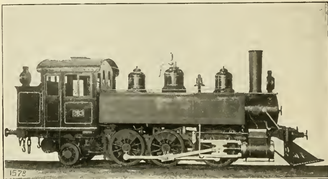
SIX COUPLED TANK LOCOMOTIVE FOR CHILE.
