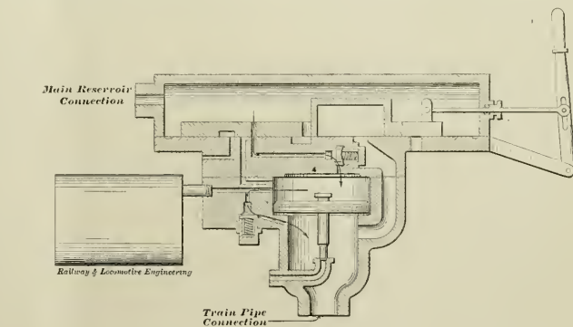
A NEWLY PATENTED BRAKE VALVE—RUNNING POSITION.
