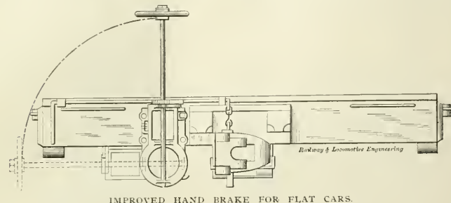
IMPROVED HAND BRAKE FOR FLAT CARS.
