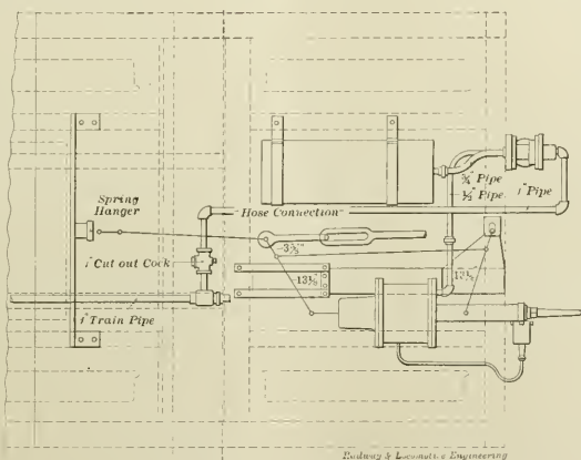
PLAIN VIEW OF DIVIDED OR TWIN BRAKE.
