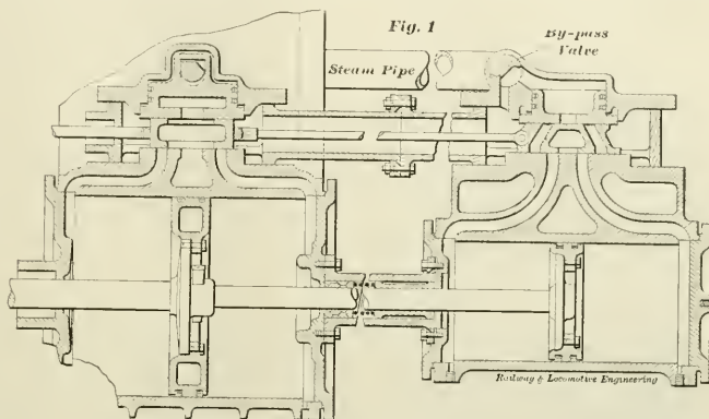
CYLINDERS OF TANDEM No. 1705 ON BALTIMORE & OHIO R. R.
