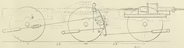
DIVIDED, OR TWIN BRAKES FOR SIX WHEEL TRUCKS.
