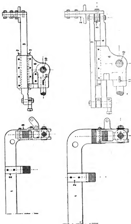
Crossheads, Guides and Guide Yokes.
