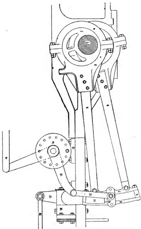
Valve Motion Work.
