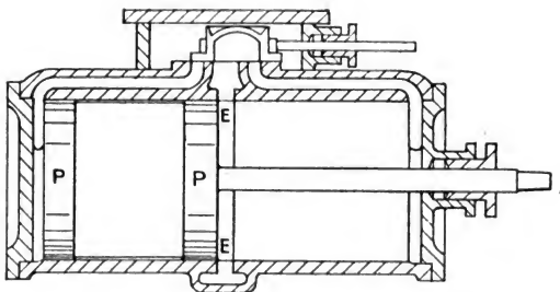
Roberts Central Exhaust, 1874.
