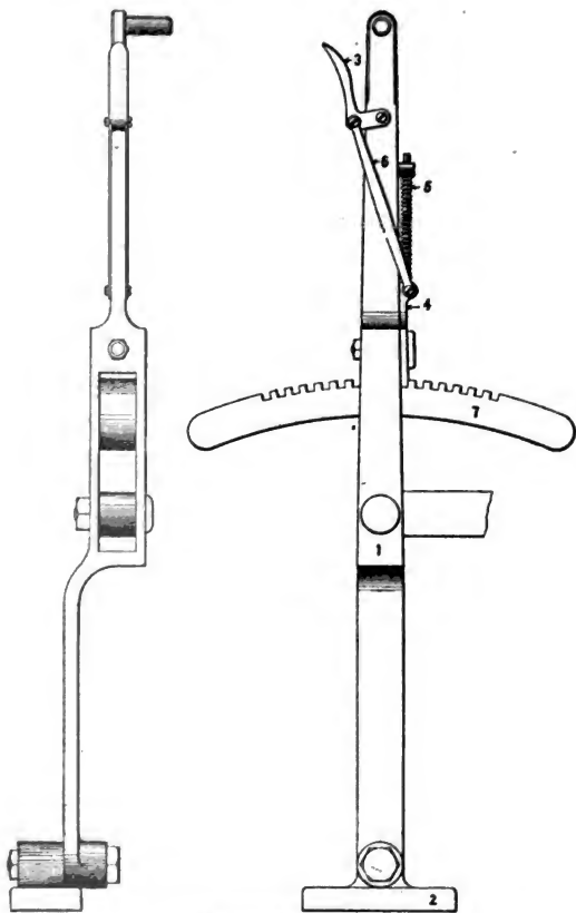
Reverse Lever.
