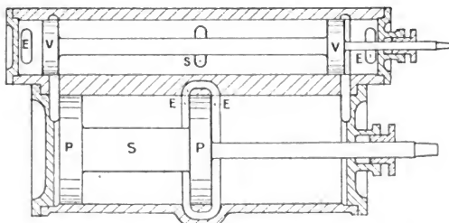
Cleveland's Central Exhaust, 1899.
