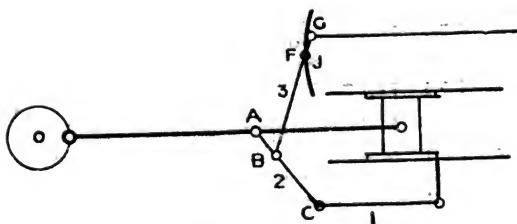
Joy Valve Gear.
