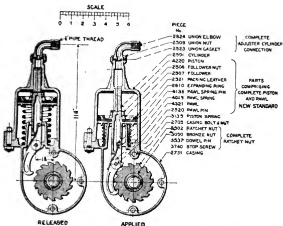
American Slack Adjuster.
