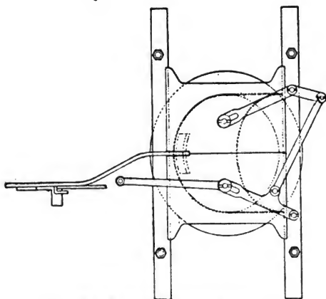
Hudson's Fire Door Deflector.
