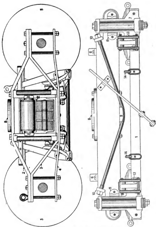
Wood Tender Truck.
