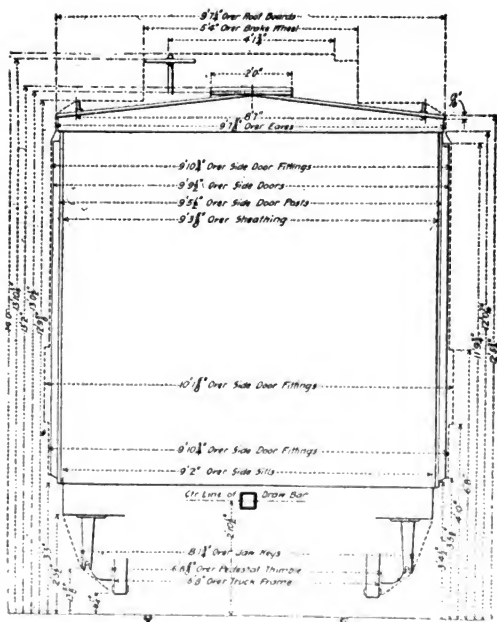
Clearance Diagram, 40-Ton Car. New York Central & Hudson River Railroad.
