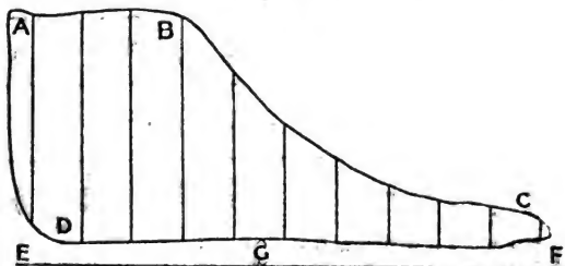
Indicator Card.
