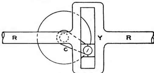
Scotch Yoke.
