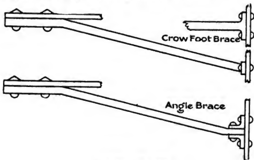
Boiler Braces.
