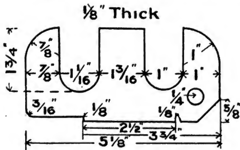
Wheel Defect Gage.
