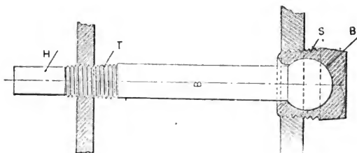
Flexible Staybolt.
