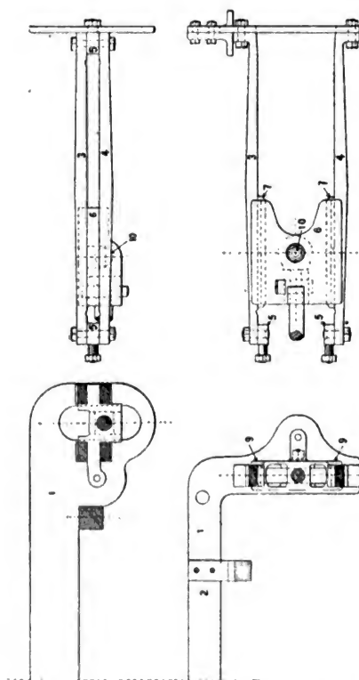
Crossheads, Guides and Guide Yokes.
