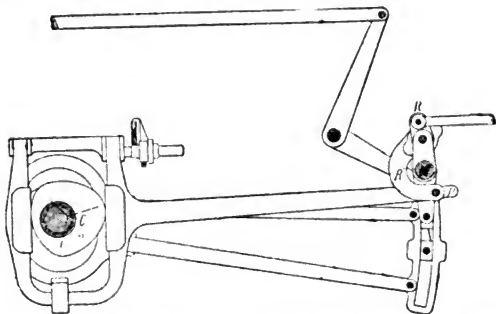
Cam Cut-off Added to Link Motion—Rogers, 1856.
