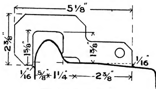
Flange Gage for Tires.
