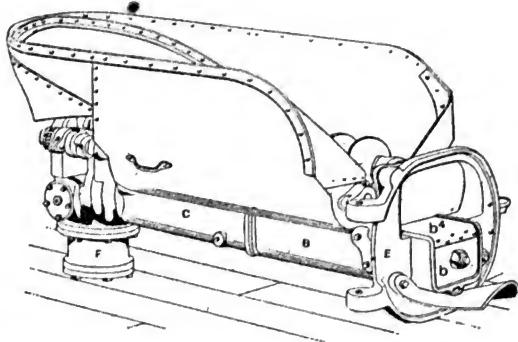
Kincaid (Victor) Mechanical Stoker.
