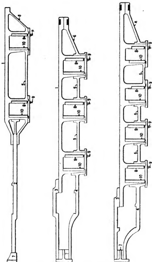
Frames of Locomotives.
