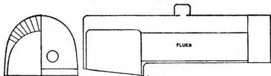
WOOTEN WIDE FIREBOX.
