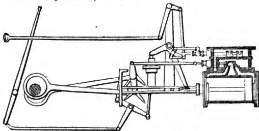
Rogers' V Hooks, Motion with Cut off.
