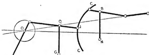
Fink Valve Gear.
