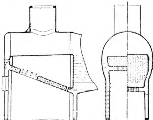
Buchanan Firebox.
