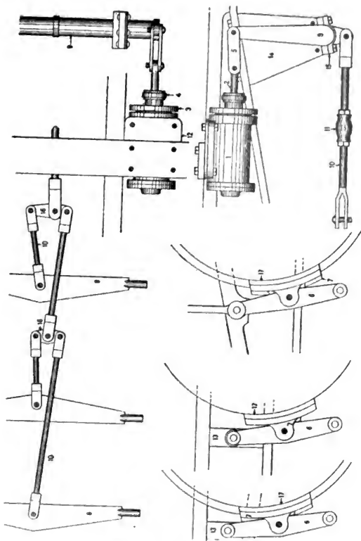
Steam Brake Work.
