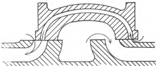
Allen Valve.
