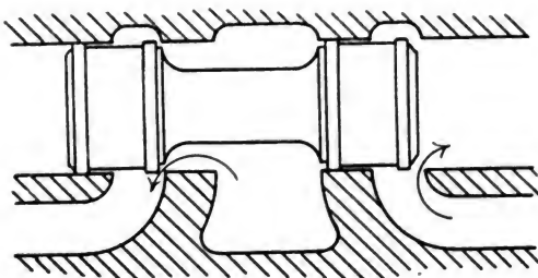
Inside Admission Piston Valve.
