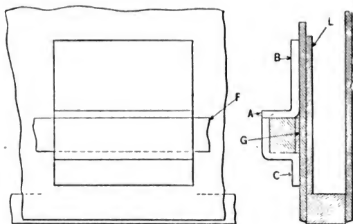
Furnace Bearer.
