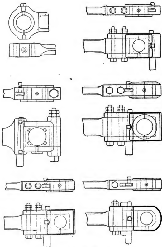
Rod Ends.
