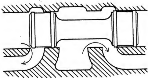
Outside Admission Piston Valve.
