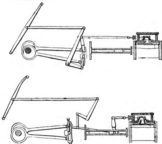
Early Link Motions.—Lower One Stationary Link (Gooch)—Rogers, 1849-1850.
